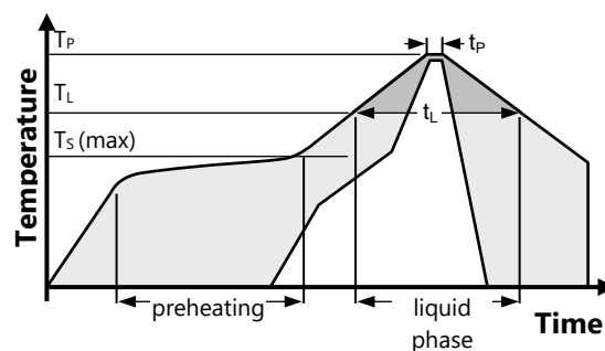
Figure 1. Soldering profile according to JEDEC standard. T_P \leq 260 \text{ °C} and t_P \leq 30 \text{ sec} above 255 \text{ °C} for Pb-free assembly. T_L < 220 \text{ °C} and t_L < 150 \text{ sec} . Ramp-up rate < 3 \text{ °C} and ramp-down rate < 6 \text{ °C/sec} for temperatures > T_L .
