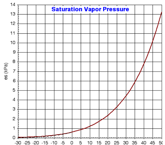
Figure 1 Saturation water vapor pressure
