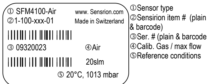
Figure 5: Label sticking on each sensor
