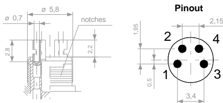
Figure 3: Connector for RS232 and power supply with pinout view from outside
